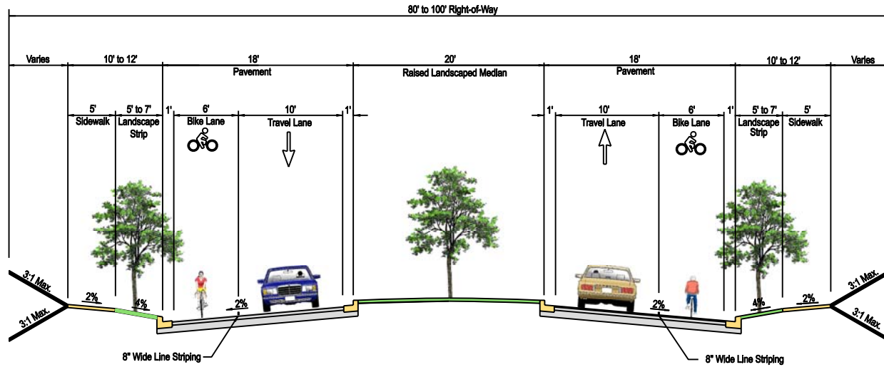
TYPICAL NORMAL SECTION - FDR BLVD.
