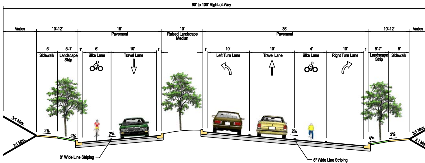
CONVENTIONAL INTERSECTION - FDR BLVD.
